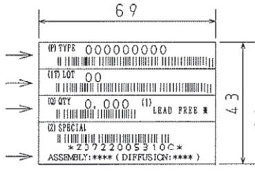
Reel label, Inner box label (unit :mm)
