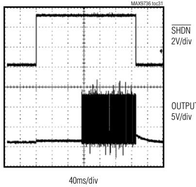
SHDN ON/OFF-RESPONSE
