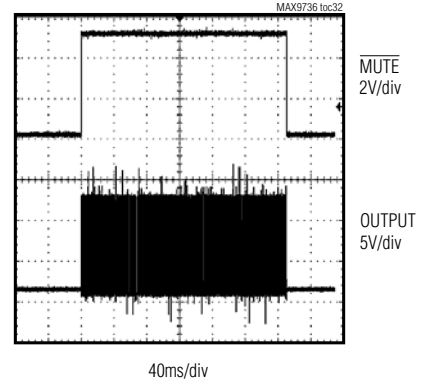
MUTE ON/OFF-RESPONSE
