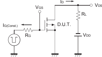
Fig.4-1 Gate charge measurement circuit
