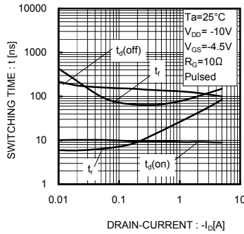
Fig.14 Switching Characteristics
