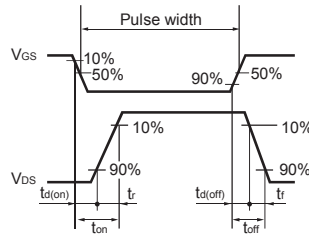
Fig.3-2 Switching waveforms
