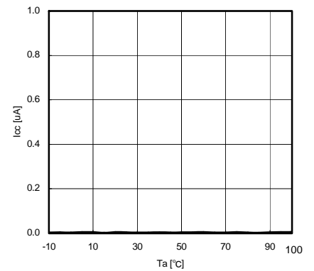
Fig.9 T_a - I_{CC} ( V_{CC}=16\text{V} , V_{EN}=0\text{V} )
