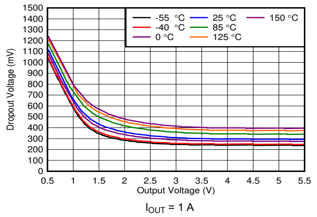
Figure 6-6. Dropout vs Output Voltage
