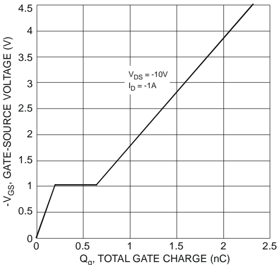
Figure 11 Gate-Charge Characteristics
