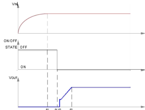
Figure 3. Startup scenario #2.
